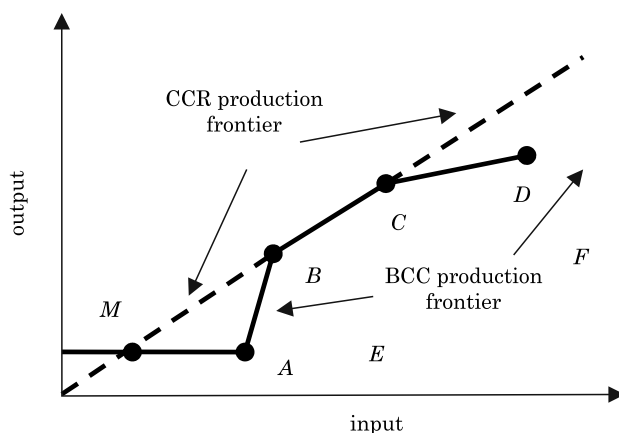
Fig. 1. Overall (CCR) and pure (BCC) technical efficiency curves
