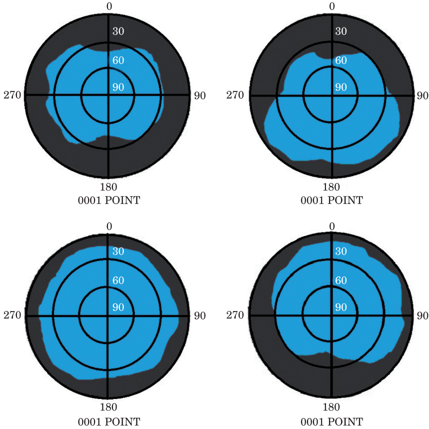
Fig. 3. The obstacles diagrams for KORTOWO points
