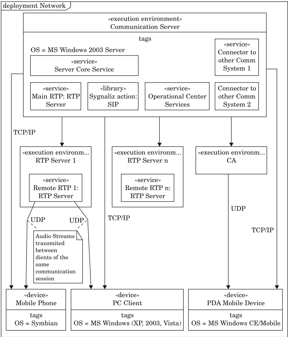
Fig. 3. SECRIKOM Silentel Server Components
