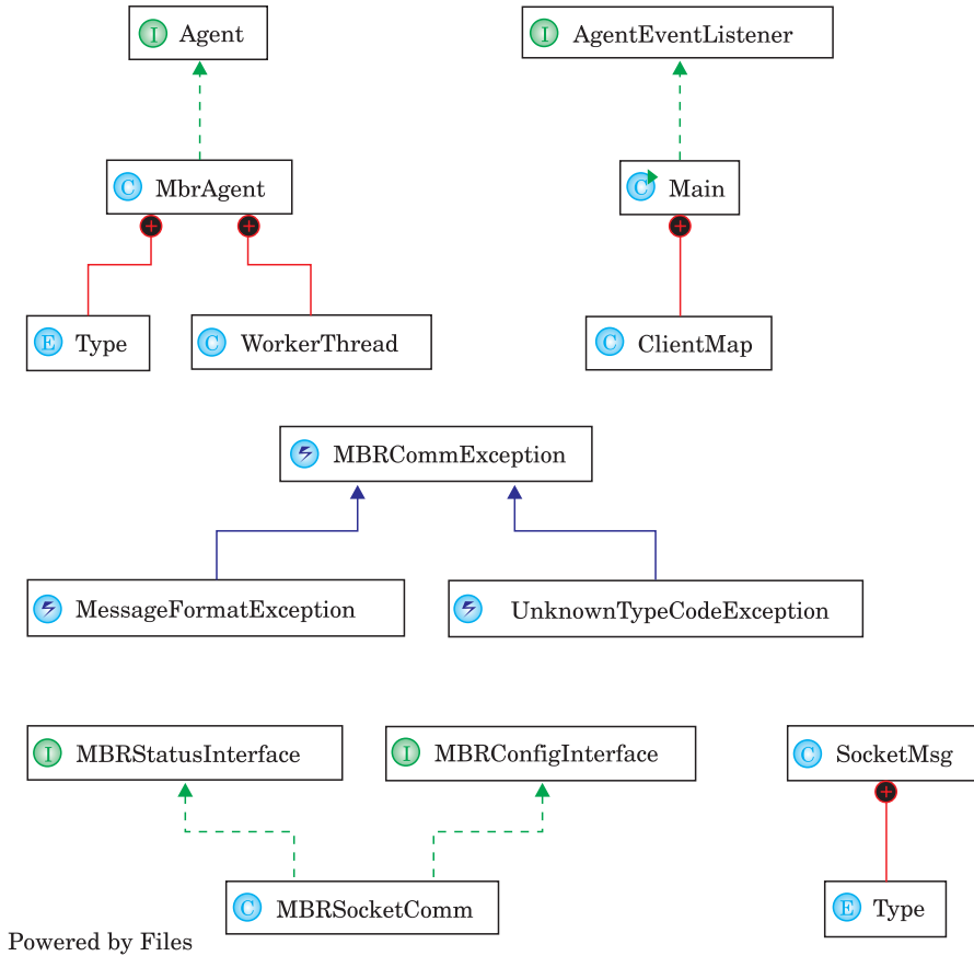
Fig. 3. The class diagram of MBR Agent implementation
