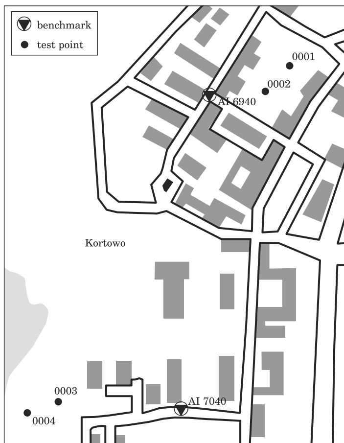
Fig. 2. The location of existing levelling benchmark and test points
