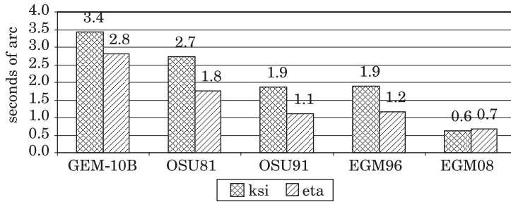
Fig. 4. Accuracy estimation of \xi \eta from the various geopotential models
